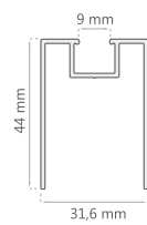
Expansor F.L. D-2018
