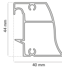
K0316 GUIA
