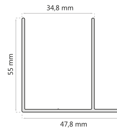
EXPANSOR D-2055
